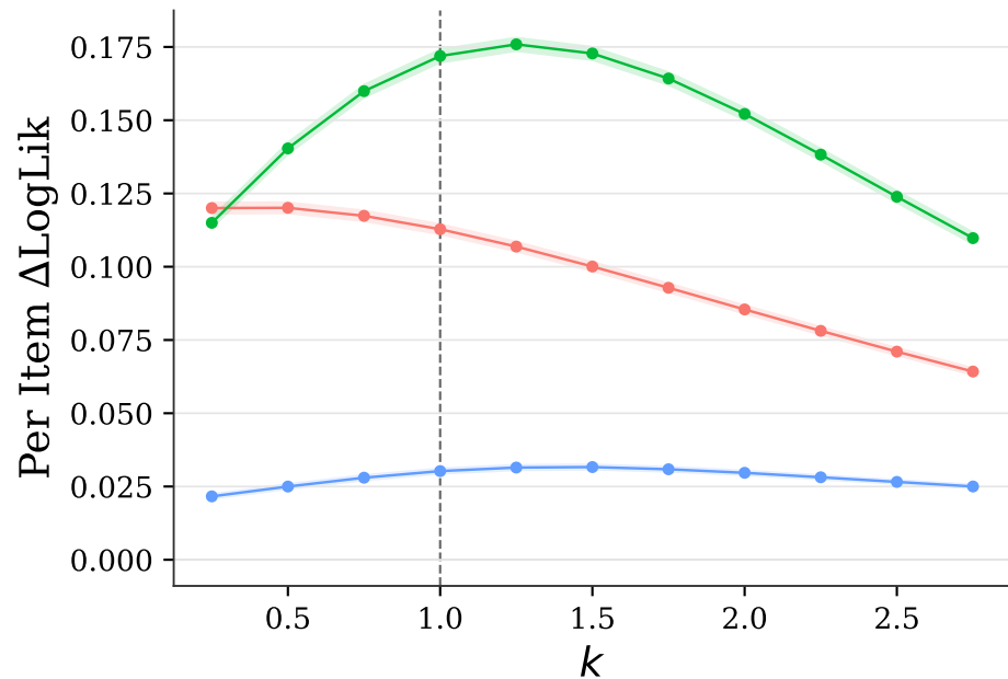
Controlled CV
