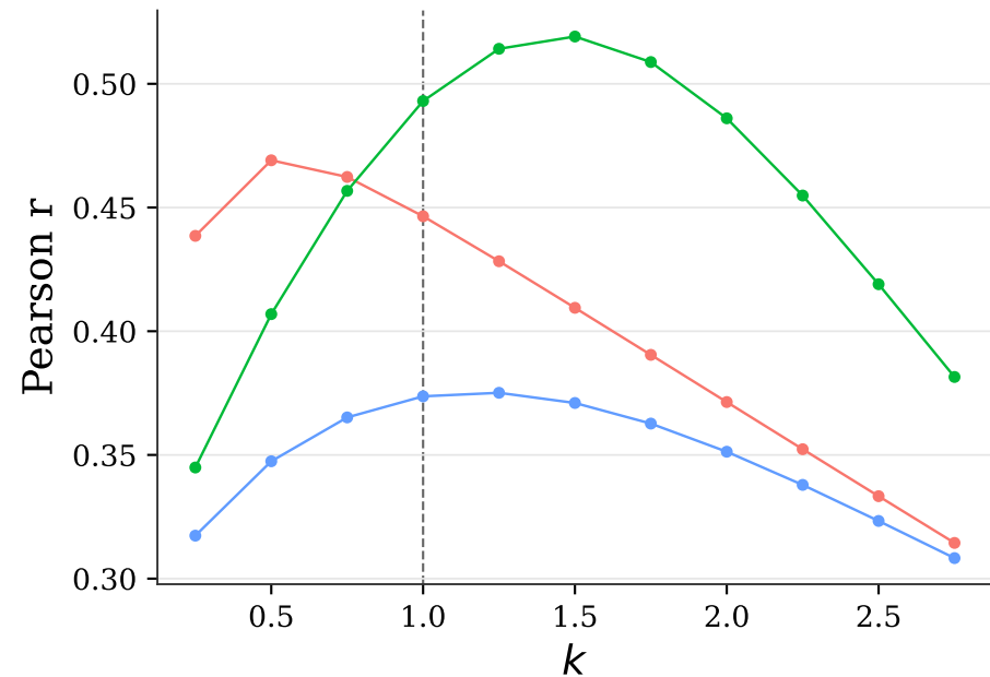
Correlation
